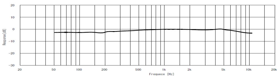
ARTIFICIAL MOUTH FREQUENCY RESPONSE (10mm)
